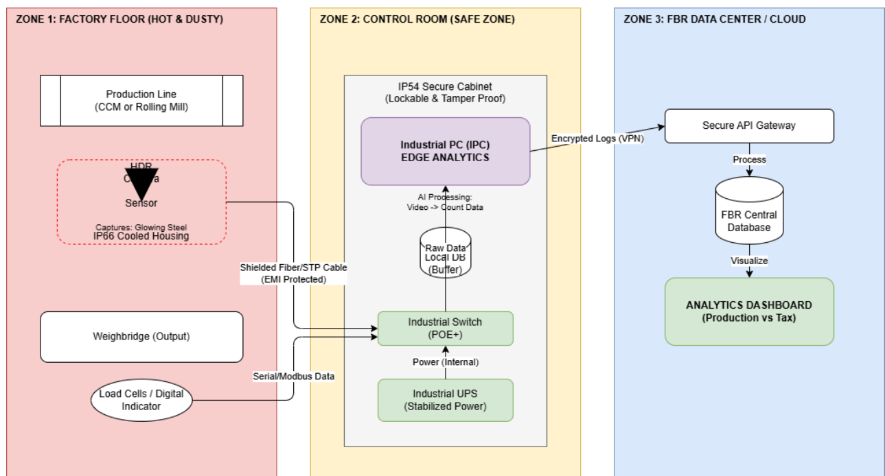
Figure A. High-level overview of technical architecture
