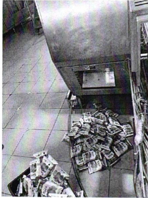
Image 13 Rejected packs discharged at the filler reject chute, upstream of the monitoring point
