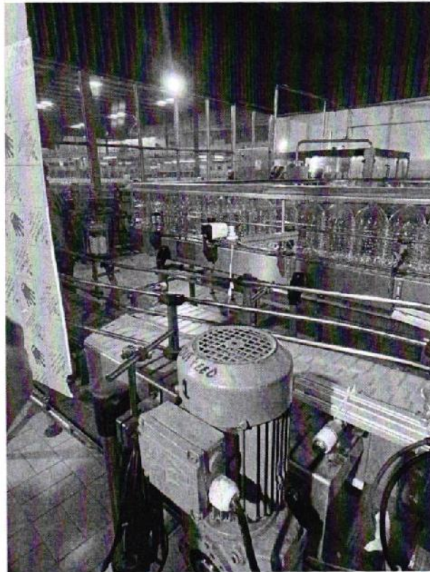
Image 4 AI vision camera (IP bullet camera) mounted over the outfeed conveyor
