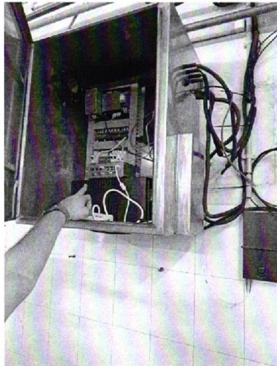
Image 2 Interior of the controller enclosure showing the PLC with I/O modules, DIN-rail power supply, terminal blocks, circuit protection, industrial edge computer, UPS and cooling fan
