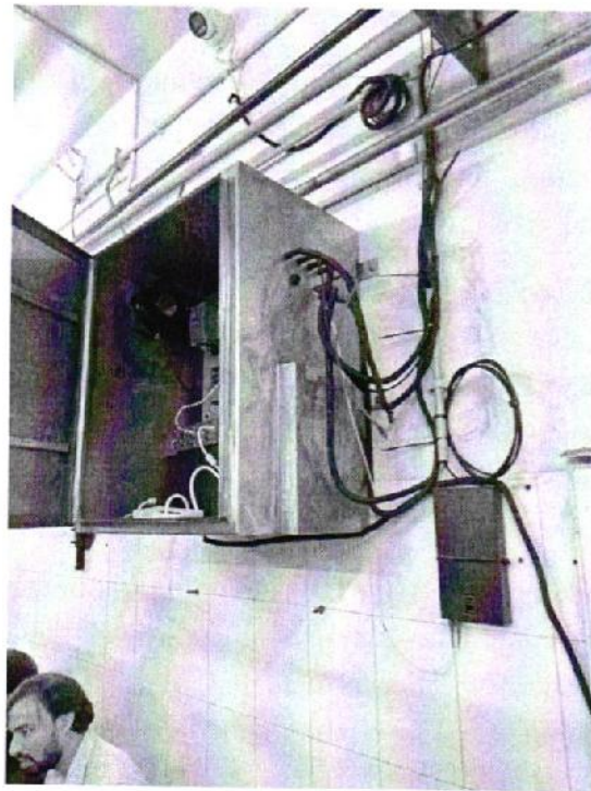
Image 1 Stainless-steel waterproof controller enclosure with the camera mounted above to monitor the barcode reading position, conduit cabling and fibre-optic termination
