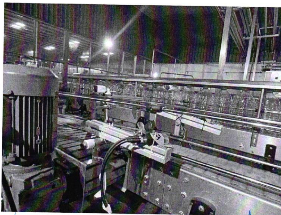
Image 2 Barcode readers positioned around the bottle conveyor for 360° reading, with aiming patterns visible on the conveyor
