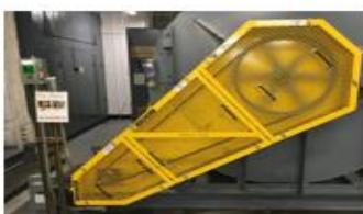
Guards for conveyor motor and belt to prevent human manipulation of counting system
