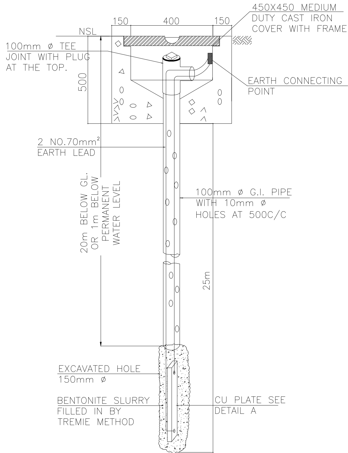
EARTH ELECTRODE
